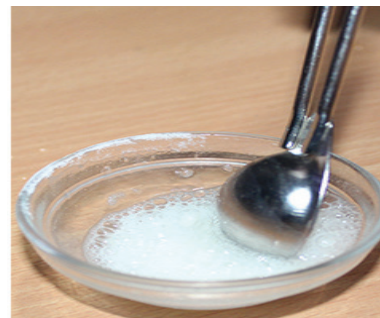
Formation of \text{CO}_2 with effervescence
