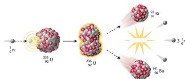
5.11 Uranium - 235 Disintegration
