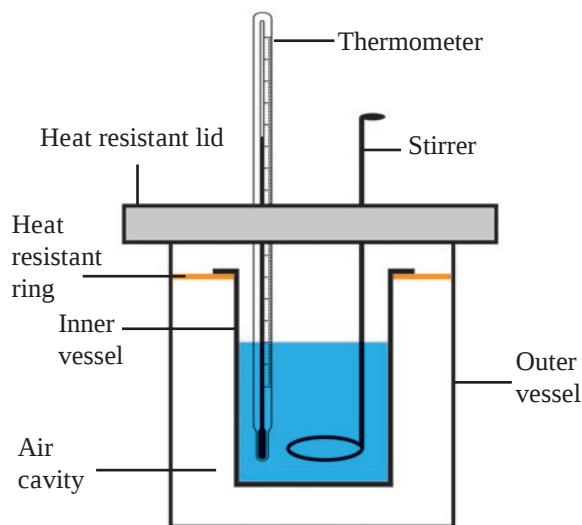
14.5 Calorimeter
